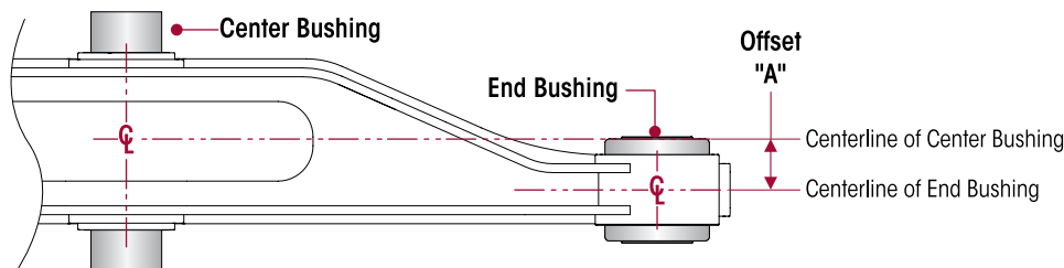
FIGURE 1 OFFSET
