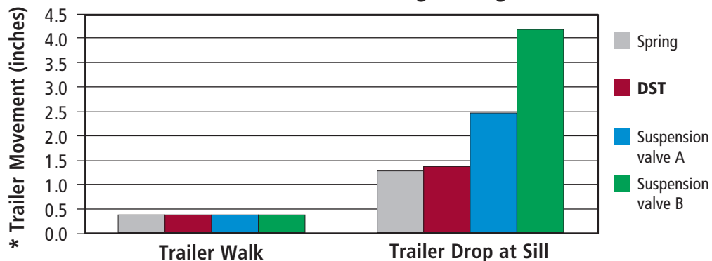
Trailer Performance During Loading
